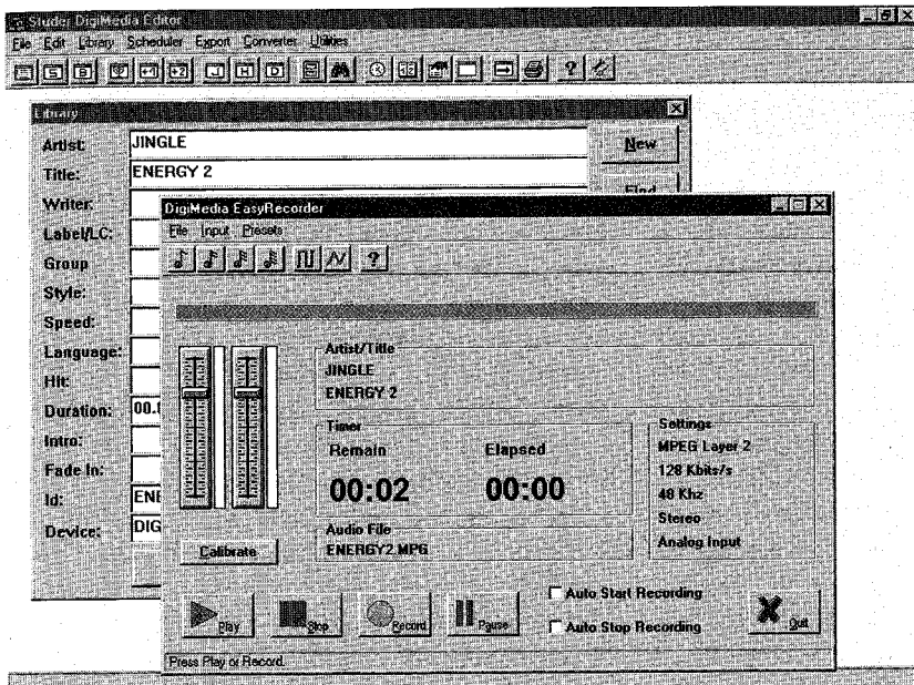
Abb. 4: Recorder/Player-Bildschirm
